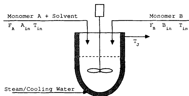
Figure 2. Semibatch reactor.
